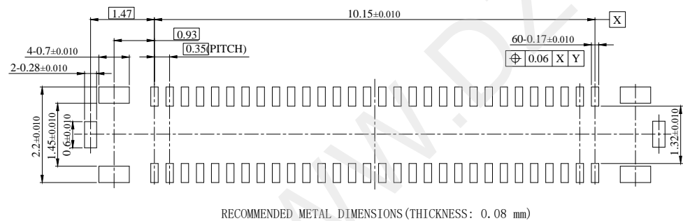
RECOMMENDED METAL DIMENSIONS (THICKNESS: 0.08 mm)
